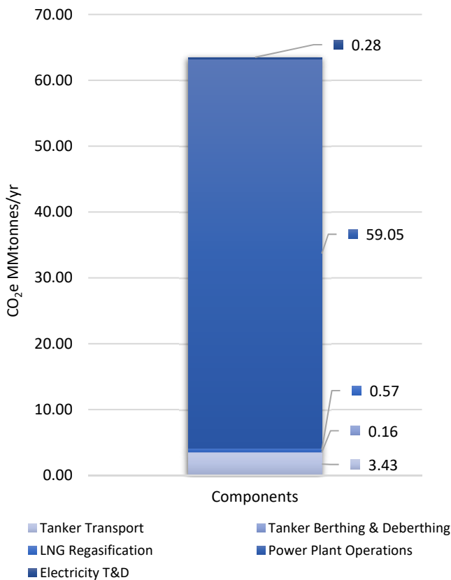
Figure 9. Downstream GHG Emissions from Alaska LNG through End Use Power Production and Distribution
