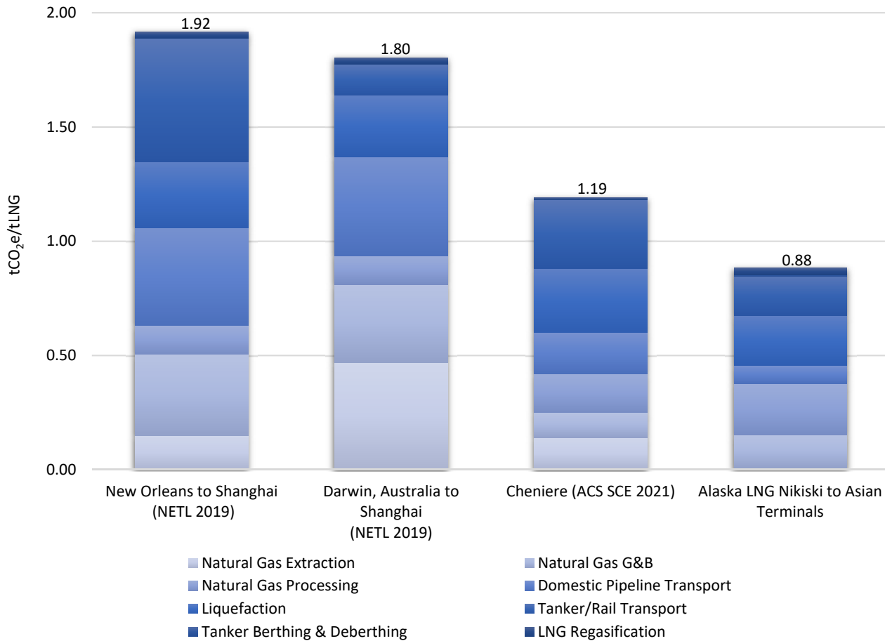
Figure 15. Natural Gas Lifecycle GHG Intensities Production through Regasification
